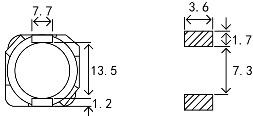
Recommended Land Pattern(mm)
