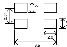
Recommended Land Pattern(mm)
