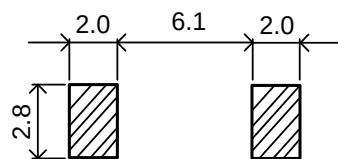
Recommended Land Pattern(mm)
