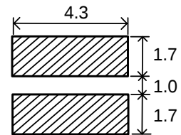
Recommended Land Pattern (mm)
