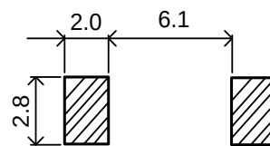
Recommended Land Pattern(mm)
