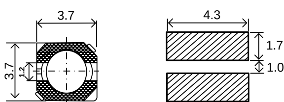
Recommended Land Pattern(mm)
