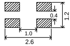
Land Pattern (mm)
