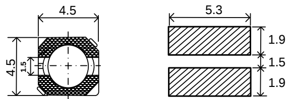
Recommended Land Pattern(mm)
