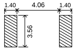
Recommended Land Pattern(mm)
