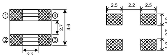
Recommended Land Pattern (mm)
