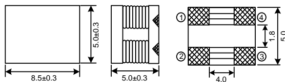
Dimensions外形尺寸 (mm)
