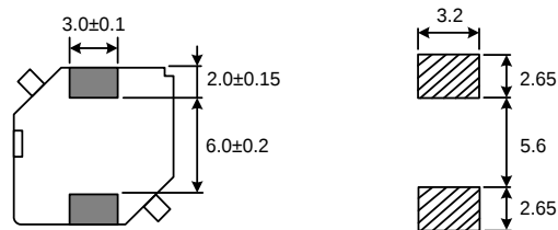
Recommended Land Pattern(mm)
