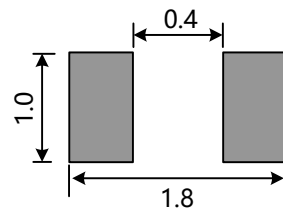
Recommended Land Pattern (mm)
