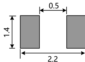
Recommended Land Pattern(mm)
