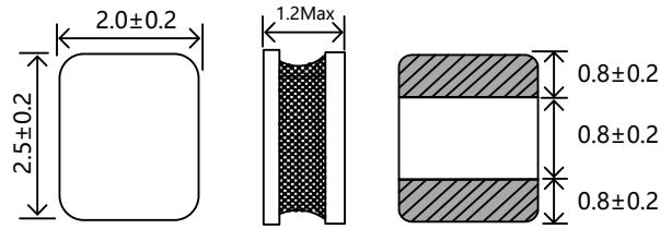
Dimensions外形尺寸 (mm)
