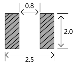
Recommended Land Pattern (mm)
